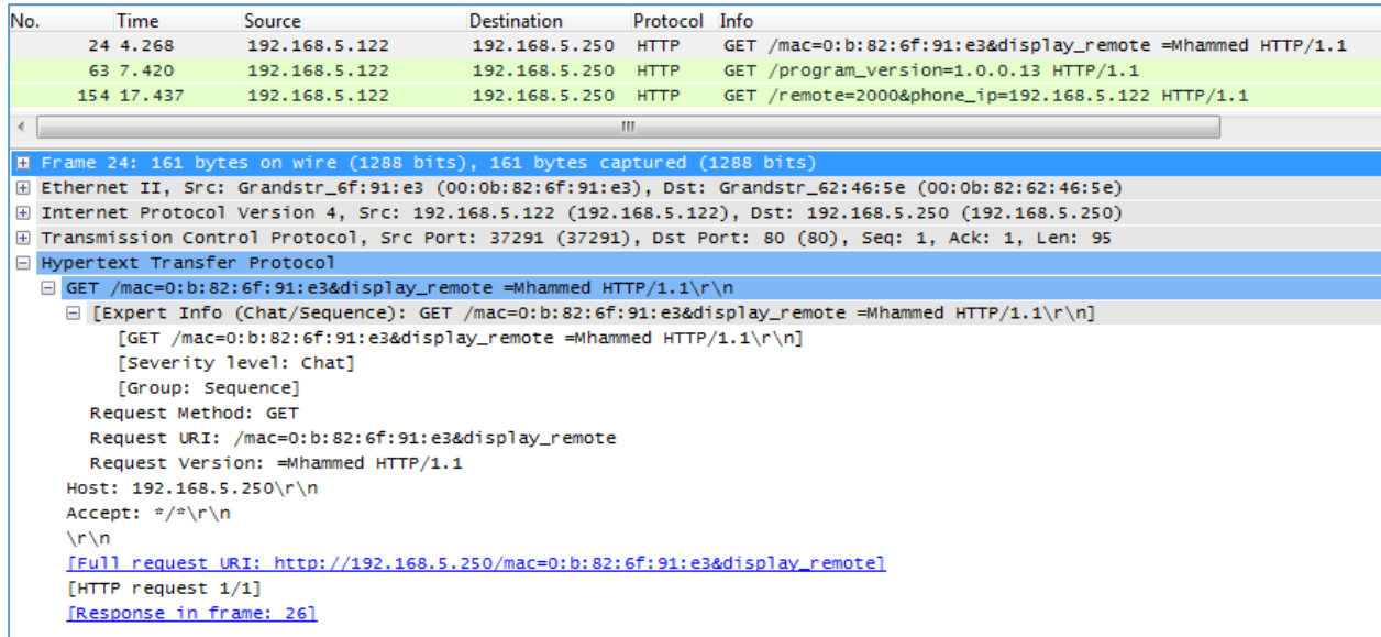
Figure 6: Action URL Packets
